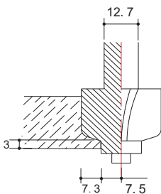
Slimline bit 1/2"Shank with bearing
